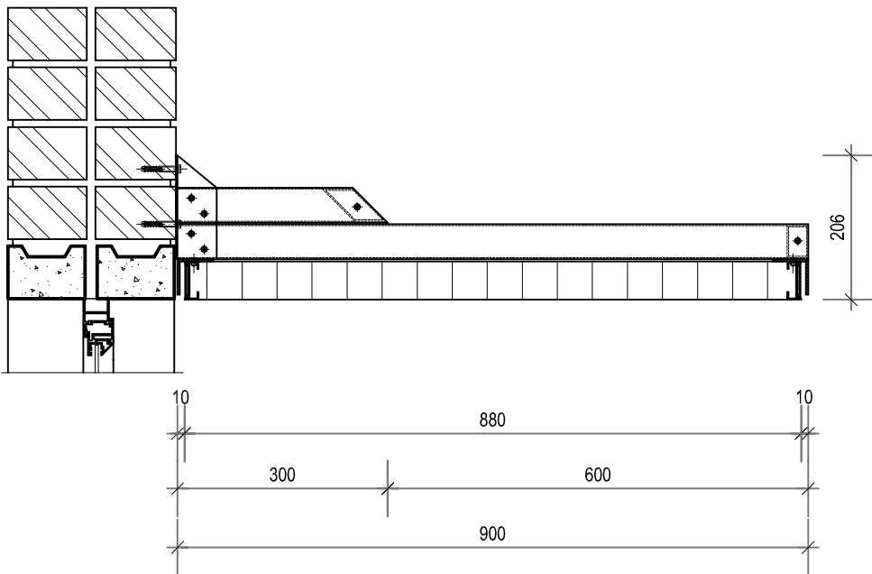
HunterDouglas FILIGREE TYPE: 1 - MODULE 50 x 50 TYPICAL SECTION PROJECTION: 900mm
