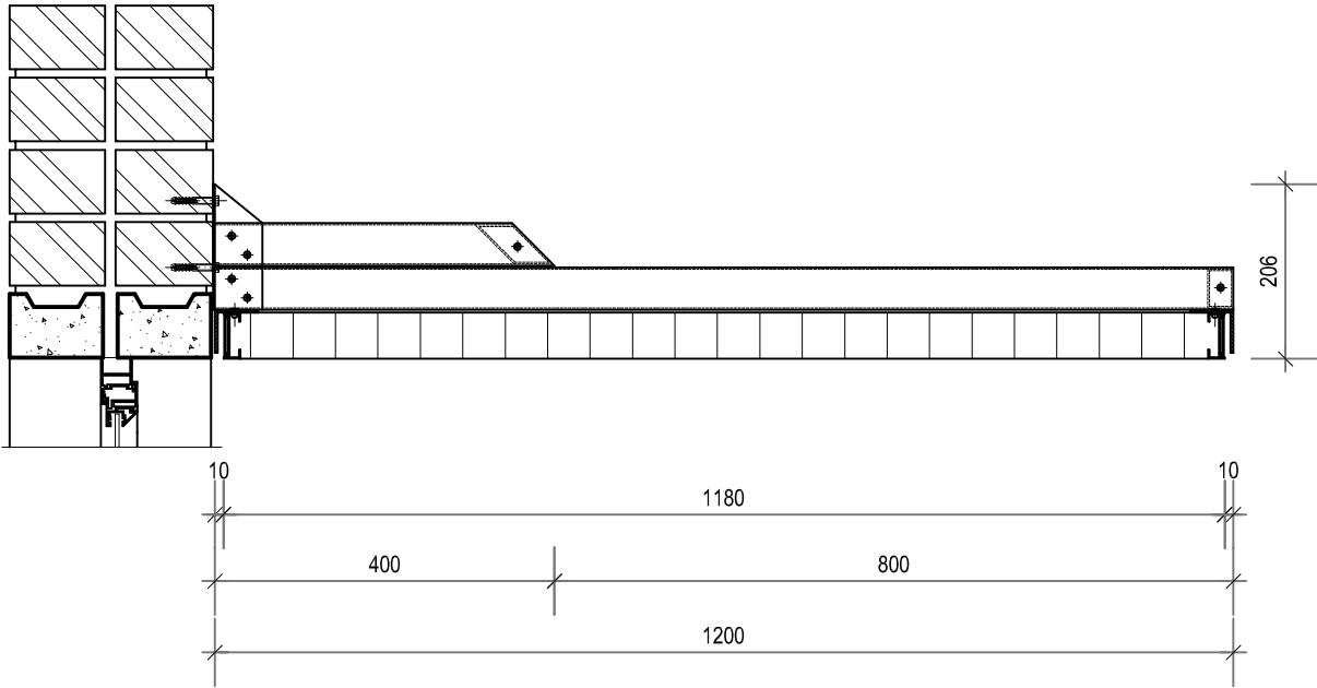
HunterDouglas FILIGREE TYPE: 1 - MODULE 50 x 50 TYPICAL SECTION PROJECTION: 1200mm
